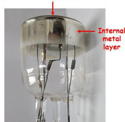
Photon-incident window with photocathode deposited inside
